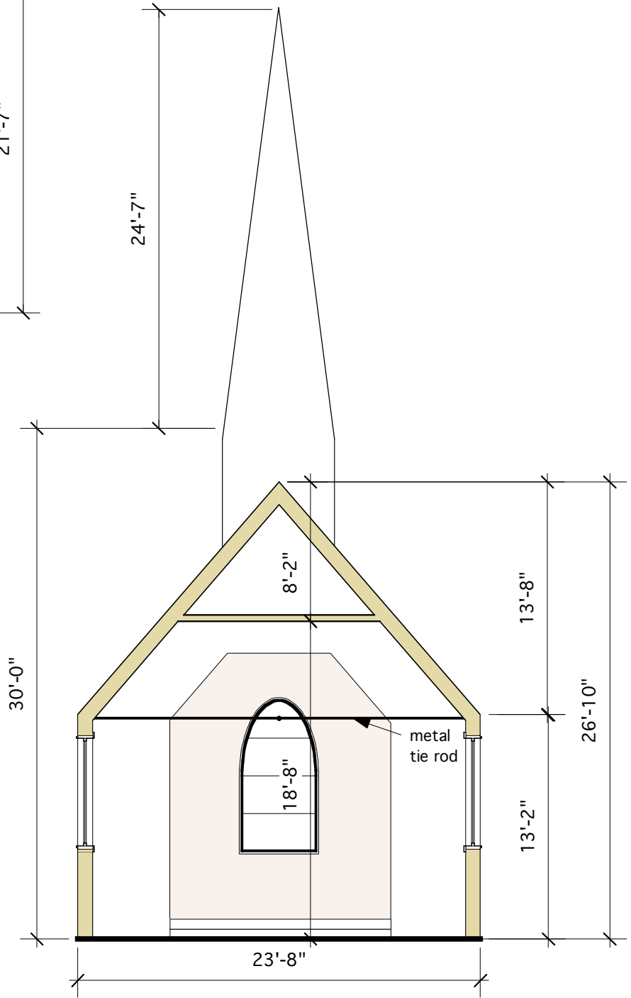
Section B-B Main Structure
