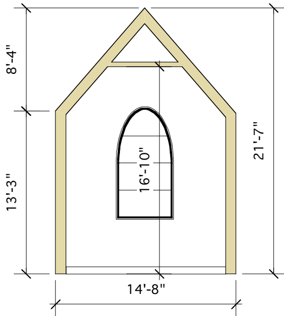
Section A-A Altar View
