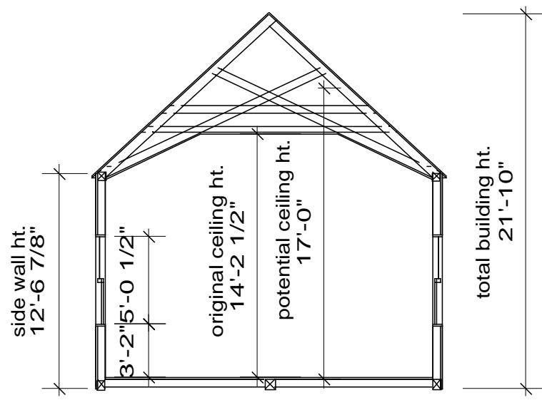
Cross-Section of Church
